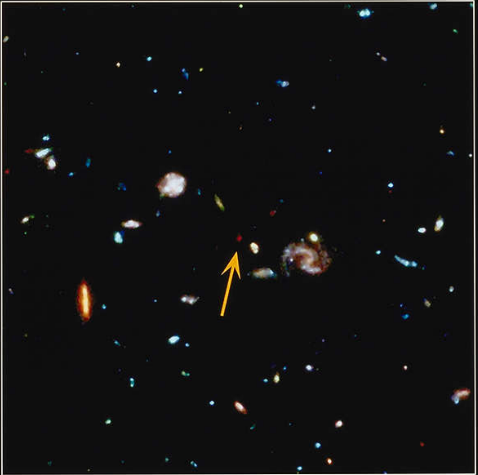
Distant Galaxy in the Hubble Deep Field - PRC98-24b - ST ScI OPO - June 26, 1996 - K. Lanzetta (SUNY Stony Brook) and NASA
